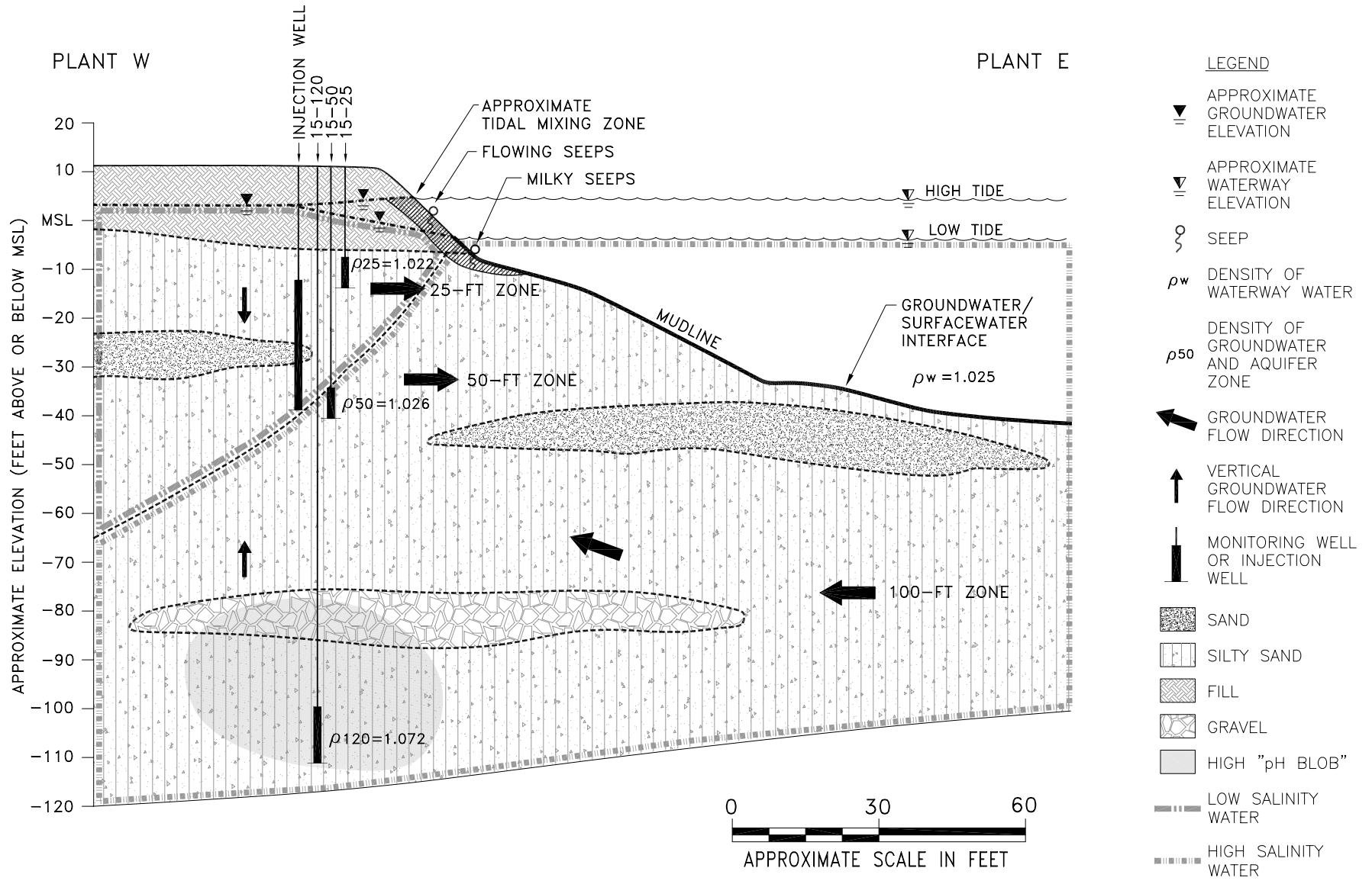
FIGURE 1-3. PLANT EAST/WEST GEOLOGIC CROSS-SECTION.
