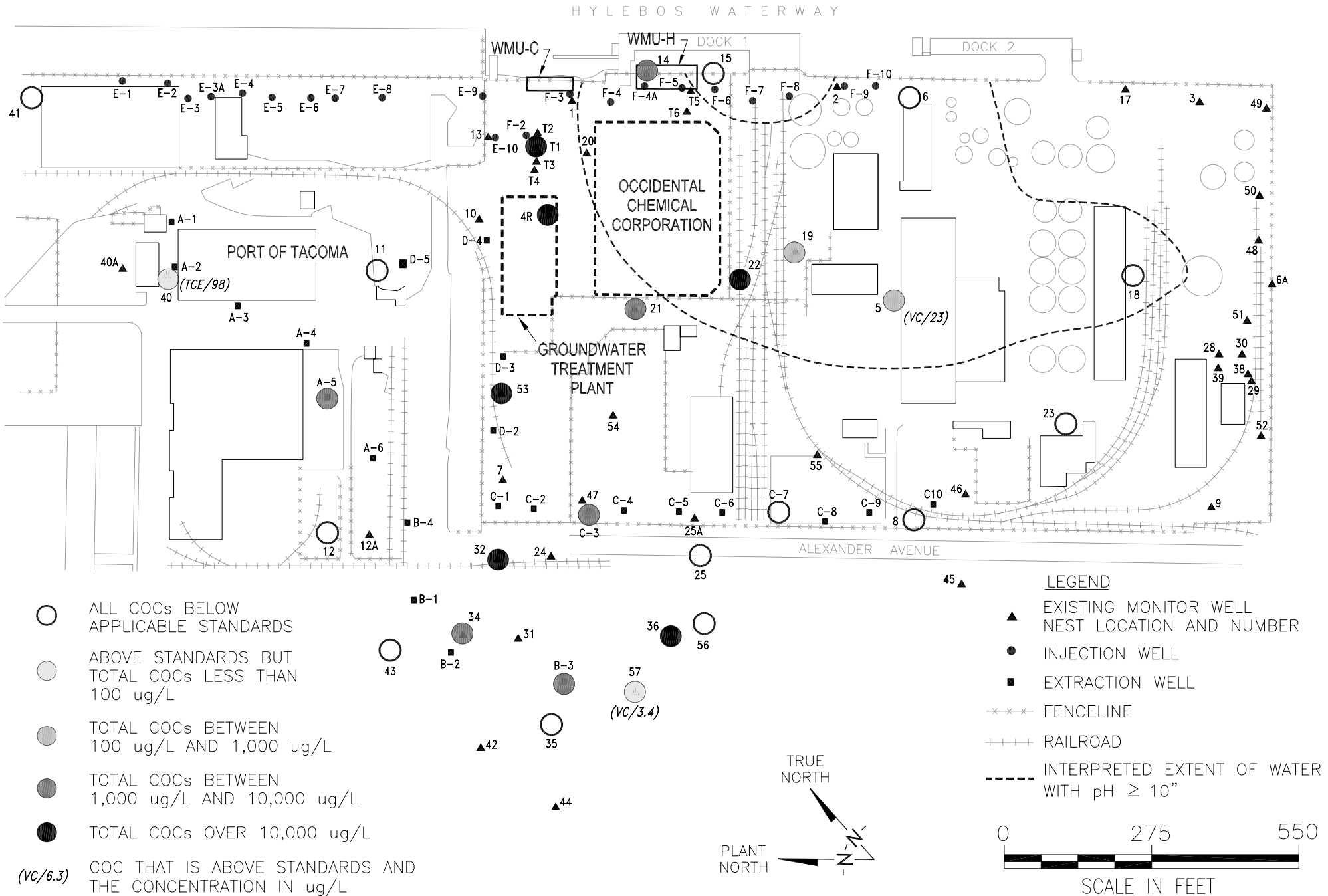
FIGURE 1-5. EXTENT OF CONTAMINATION AT 50 FEET BELOW GROUND SURFACE - AUGUST 2002
