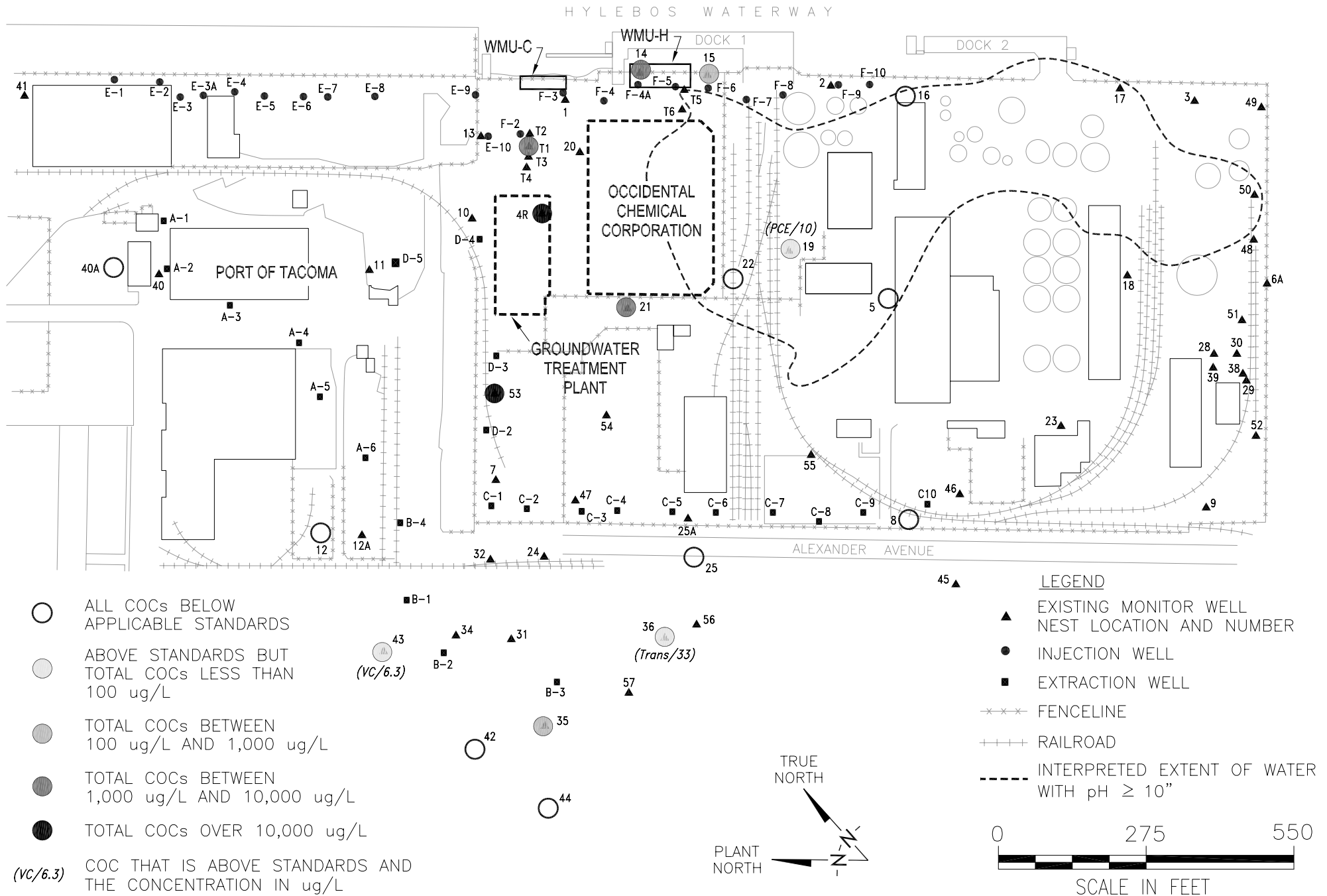
FIGURE 1-4. EXTENT OF CONTAMINATION AT 25 FEET BELOW GROUND SURFACE - AUGUST 2002
