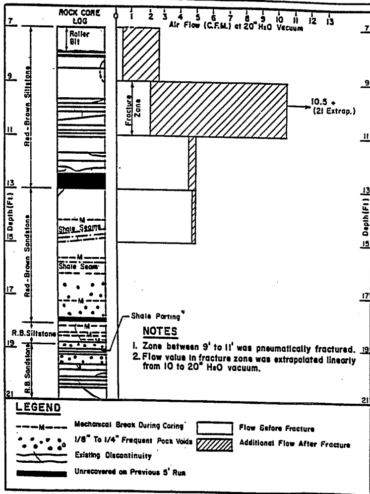
Figure D-1. Air permeability log, 9-11 ft fracture zone.
