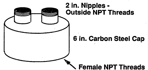
Figure A-2. Wellhead design.
