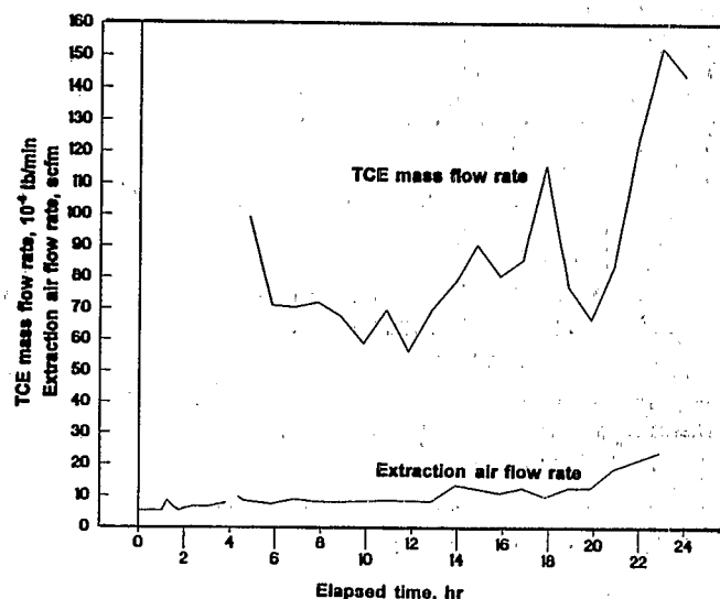
Figure C-7. TCE mass removal rates, 24-hr HGI test.
