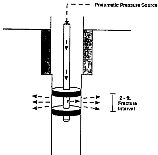
Figure A-1. HQ Injector.
