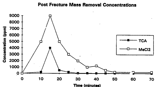
Figure D-3. Effect of fracturing, Richmond, VA site.
