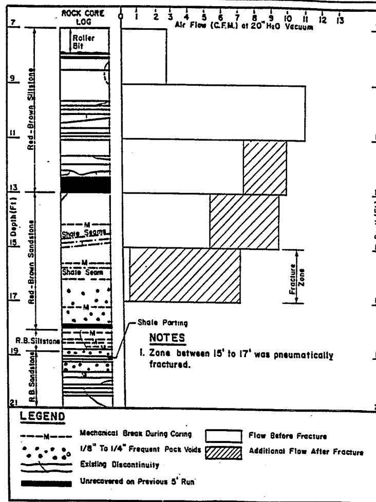
Figure D-2. Air permeability log, 15-17 ft fracture zone.
