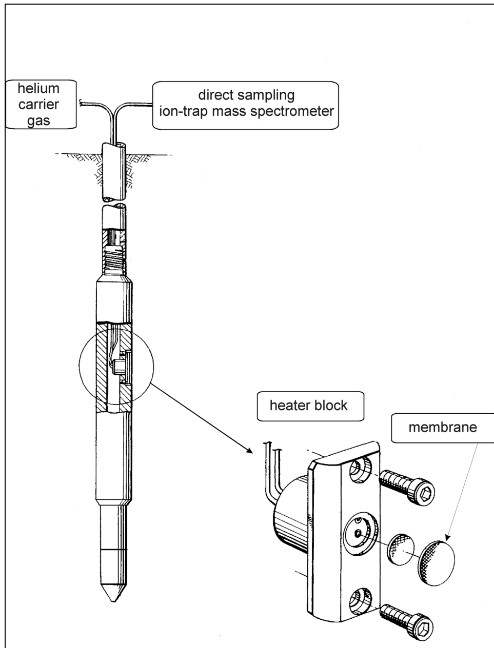
Figure 2. Combined Probe (courtesy of Geoprobe Systems, Salina, KS, from Christy 1997)
