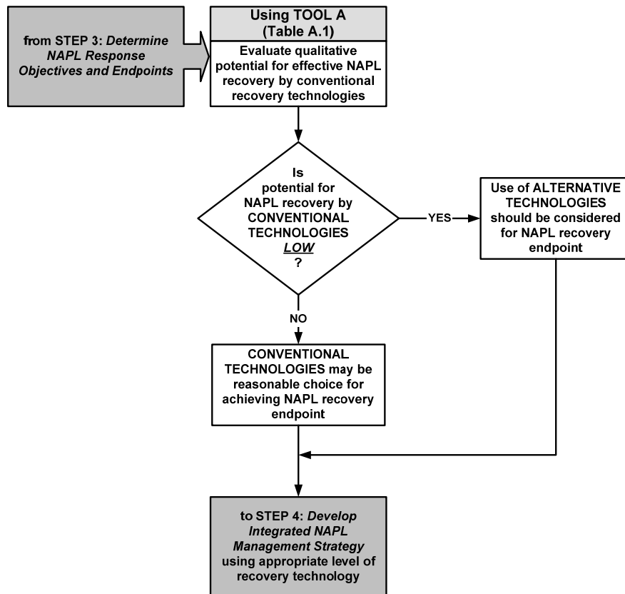
Figure A.1. Use of TOOL A: Screen for Potential of Conventional NAPL Recovery Technology
