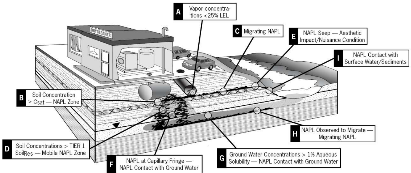
Figure E.1. Results of NAPL Assessment for Example Problem 2.
