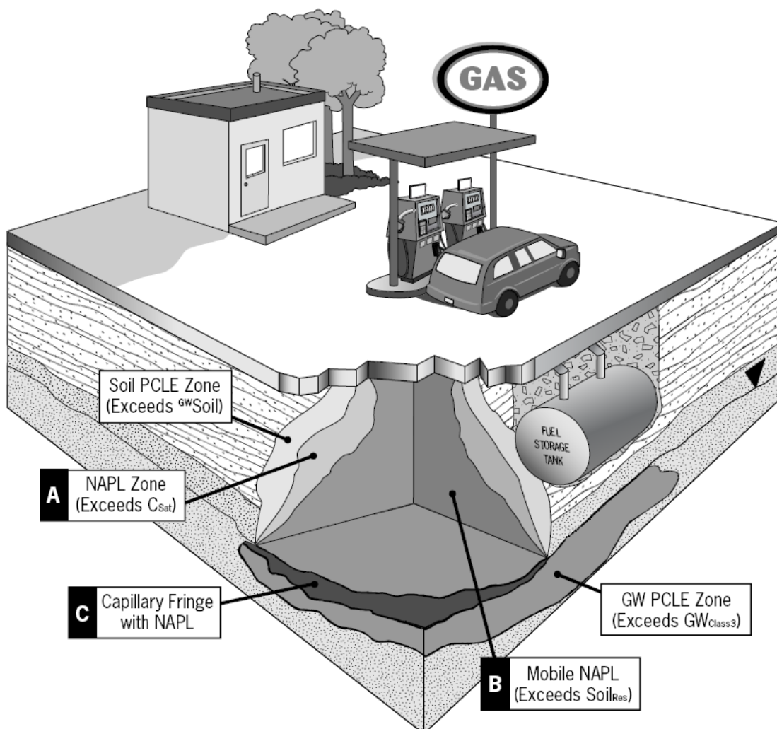
Figure D.1. Results of NAPL Assessment for Example Problem 1.
