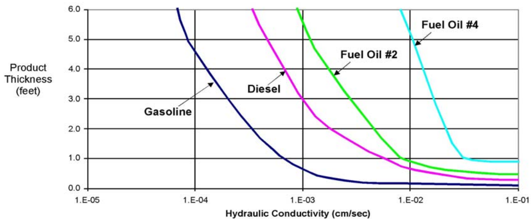
Figure C.1. Example Quantitative Screen for Conventional NAPL Recovery System (EXAMPLE: NOT FOR ACTUAL USE. SITE-SPECIFIC MODELS MUST BE DEVELOPED.)
