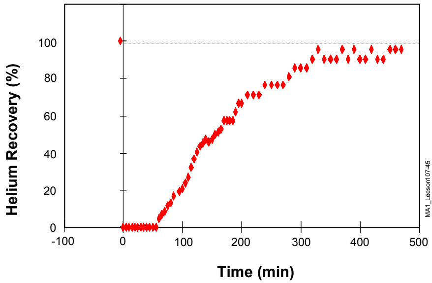
Figure 3. Helium Recovery at an Extraction Rate of 80 scfm and (A) an Air Injection Rate of 5 scfm and (B) an Air Injection Rate of 10 scfm, Port Hueneme, CA
