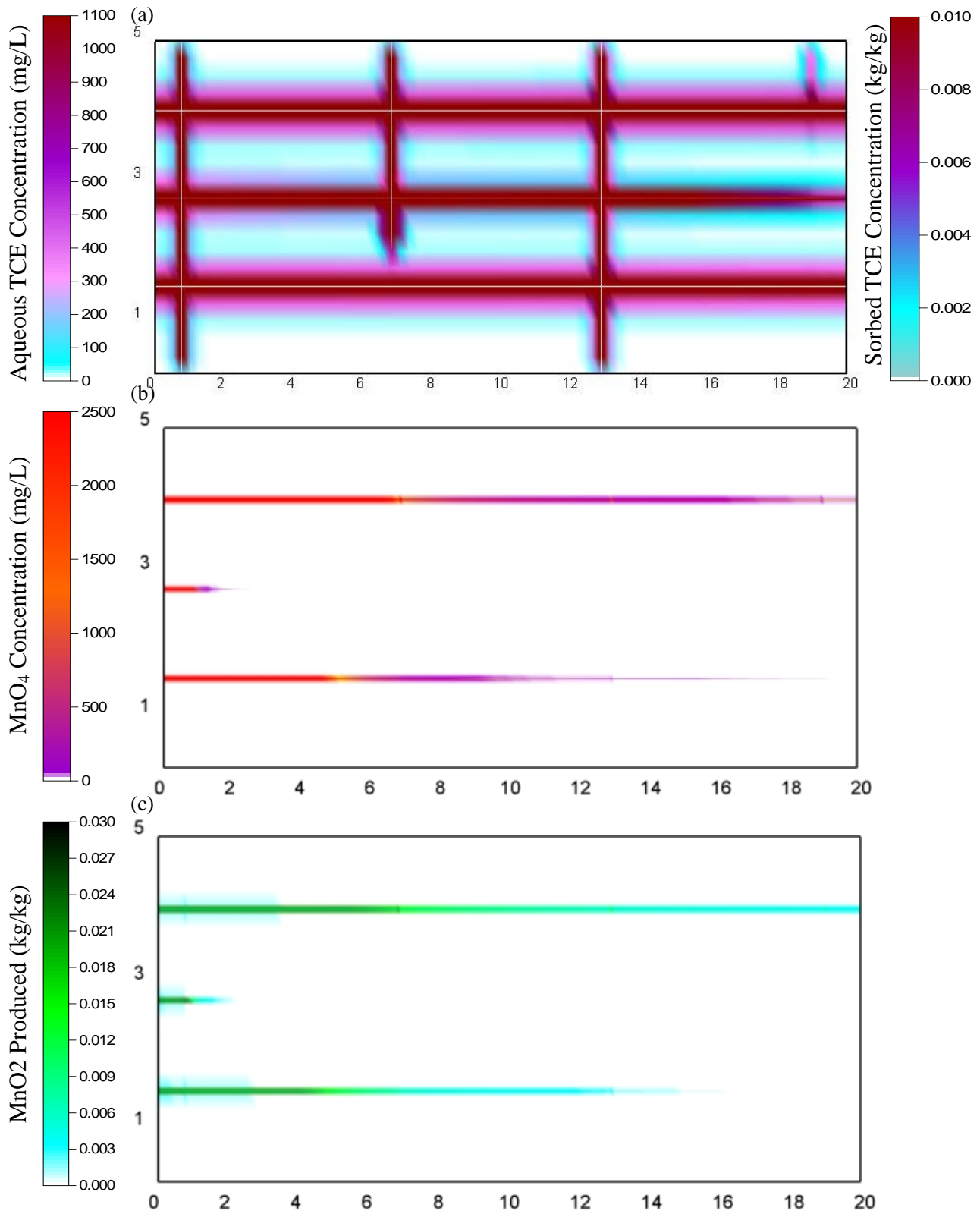
Figure A2: Distribution of aqueous species concentrations at t_{\text{TOTAL}} = 23 years for 1250 mg/L of MnO 4 Simulation, after 2 years of chemical oxidation (i.e., Treatment stage): (a) TCE, (b) MnO 4 , (c) MnO 2
