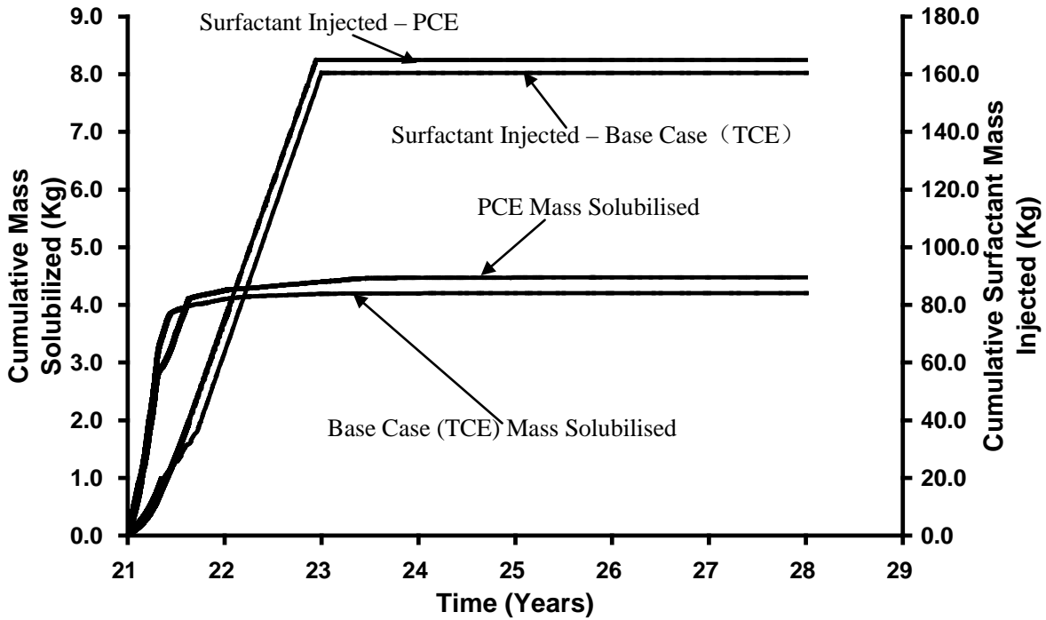
Figure 24: Comparison of cumulative mass solubilised by micelles and surfactant injected for period between 21 to 28 years.
