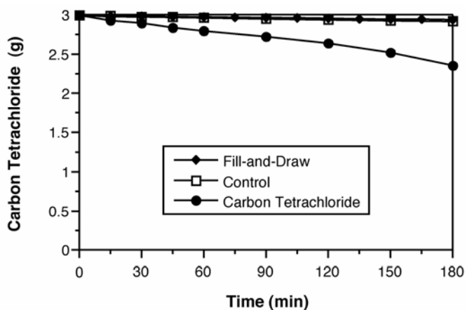
Figure 8.4.1-2. \text{MnO}_2 -catalyzed CHP destruction of 3.0 g CT DNAPL. (Reaction conditions: 1 g \text{MnO}_2 , 294 mM steady state \text{H}_2\text{O}_2 , pH 7; T = 20 \pm 2 \text{ }^\circ\text{C} ).
