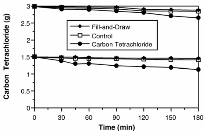
Figure 8.4.1-1. CHP destruction of 3.0 g and 1.5 g CT DNAPLs. (Reaction conditions: 5 mM \text{Fe}_2(\text{SO}_4)_3 , 1470 mM steady state \text{H}_2\text{O}_2 , pH 3; T = 20 \pm 2 \text{ }^\circ\text{C} )
