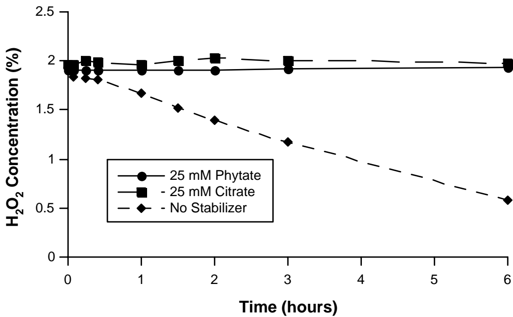
Figure 8.6.6-2. Rate of stabilized and unstabilized H 2 O 2 decomposition in a column of manganese coated sand (MCS).
