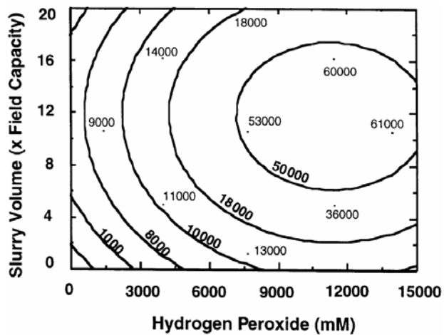
Figure 8.3.3-5. Benzo[ a ]pyrene oxidation stoichiometry in the Palouse loess as a function of H 2 O 2 concentration and slurry volume at pH 8.0. Isoconcentration lines represent the moles H 2 O 2 consumed/ 14 C-CO 2 described by equation 8.
