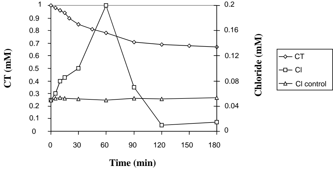
Figure 8.2.2-14. Chloride release with CT degradation
