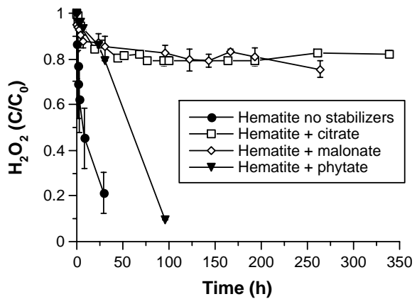
Figure 8.6.5-2. Decomposition of hydrogen peroxide in hematite slurries at pH 3 without stabilization or with addition of 10 mM citrate, malonate, or phytate
