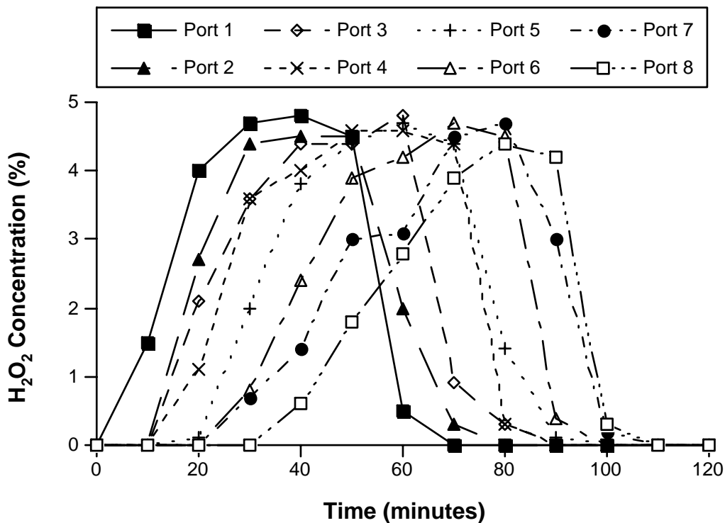
Figure 8.6.6-7. Decomposition of H 2 O 2 stabilized by 25 mM citrate in a column of manganese coated sand (MCS) at pH 7.
