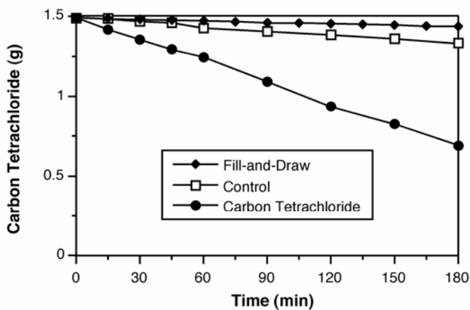
Figure 8.4.1-3. \text{MnO}_2 -catalyzed CHP destruction of a 1.5 g CT DNAPL. (Reaction conditions: 1 g \text{MnO}_2 , 294 mM steady state \text{H}_2\text{O}_2 , pH 7; T = 20 \pm 2 \text{ }^\circ\text{C} ).
