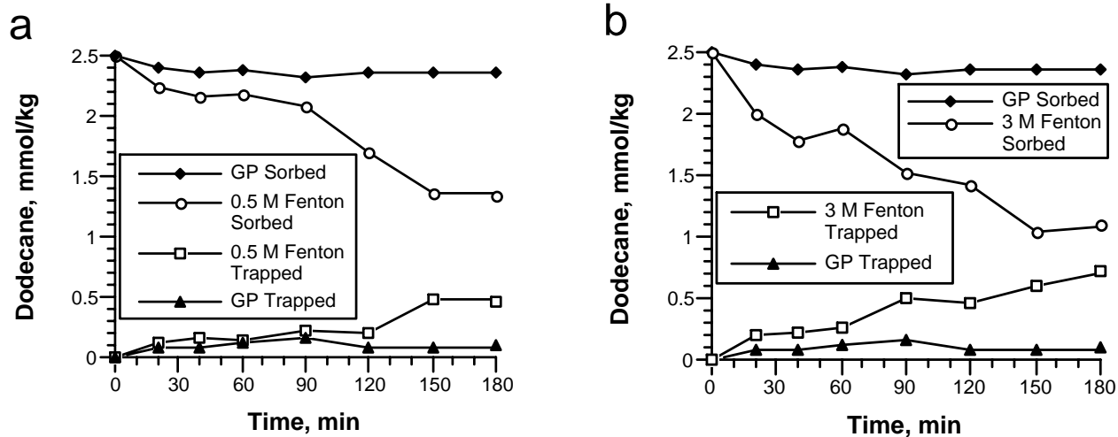
Figure 8.5.2-2. Desorption of dodecane by a CHP reaction: a) 0.5 M H 2 O 2 ; b) 3 M H 2 O 2 (experimental reactors: 50 g of silica sand spiked with dodecane at 2.5 mmol/kg sand; 5 mM Fe(III) and 0.5 M or 3 M H 2 O 2 ; 50 ml total volume at pH 3.0; control reactors: H 2 O 2 substituted by deionized water; T = 20 ± 2°C).
