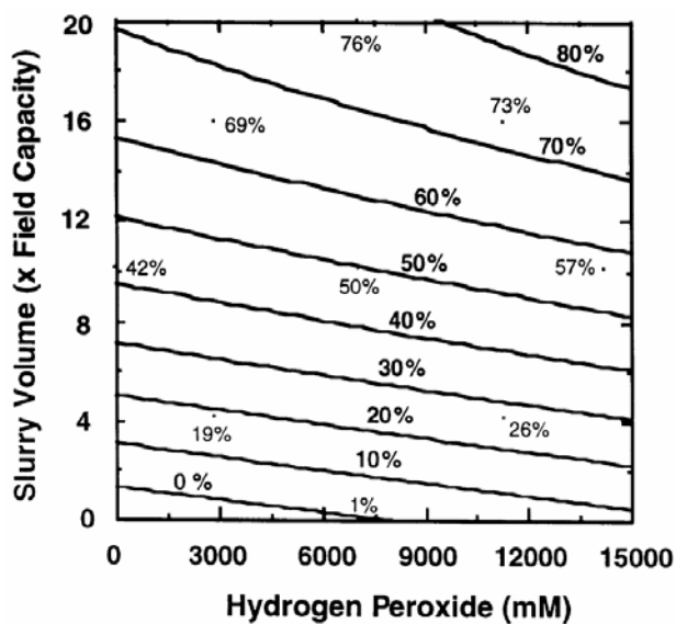
Figure 8.3.3-4. Response surface for the mineralization of 14 C-BaP as a function of H 2 O 2 concentration and slurry volume in Palouse loess catalyzed by naturally occurring iron oxyhydroxides at pH 8. Isoconcentration lines represent the per cent BaP recovered as 14 C-CO 2 described by equation 7. The field capacity of the Palouse loess = 0.42 ml/g.
