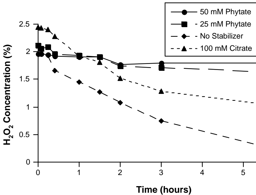
Figure 8.6.6-1. Rate of stabilized and unstabilized H 2 O 2 decomposition in a column of iron coated sand (ICS).
