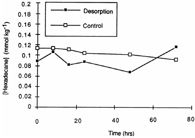
Figure 8.3.4-1. Desorption of 0.1 \text{ mmol kg}^{-1} hexadecane from silica sand.
