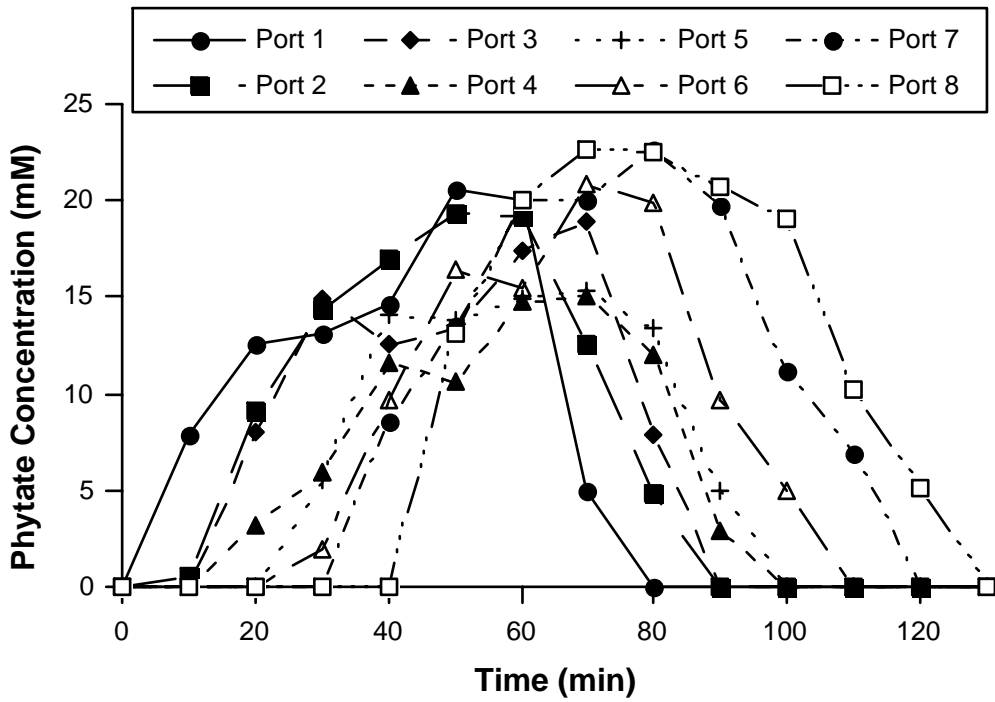
Figure 8.6.6-17. Concentration of phytate in each of eight ports over time in a column of iron coated sand (ICS) containing hexachlorobenzene (HCB) treated with H 2 O 2 stabilized by 25 mM phytate at pH 7.
