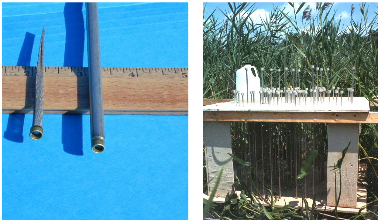
Figure 20. Photographs of tubing and screen components of tubing sampler (left) and the tubing sampler array at wetland field site (right). USGS photos
