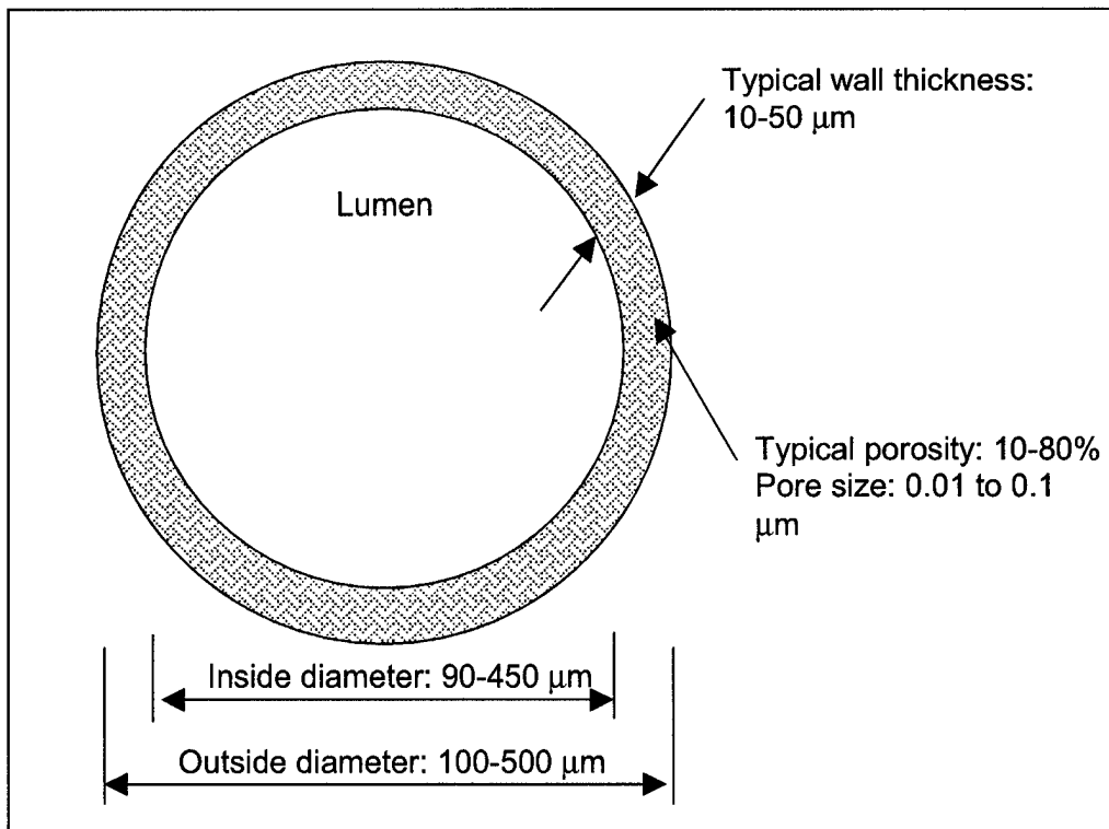
Figure 4-3. HFM cross-section.
