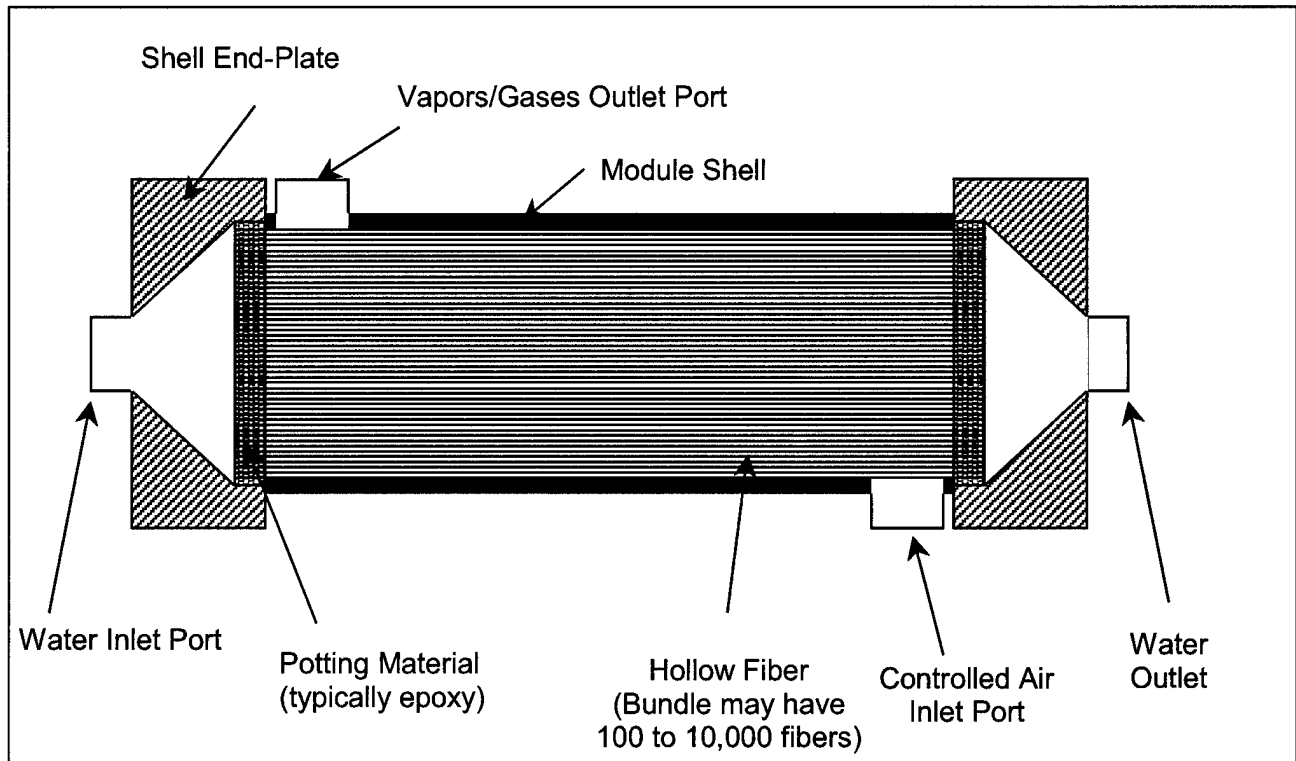
Figure 4-4. HFM flow schematic.
