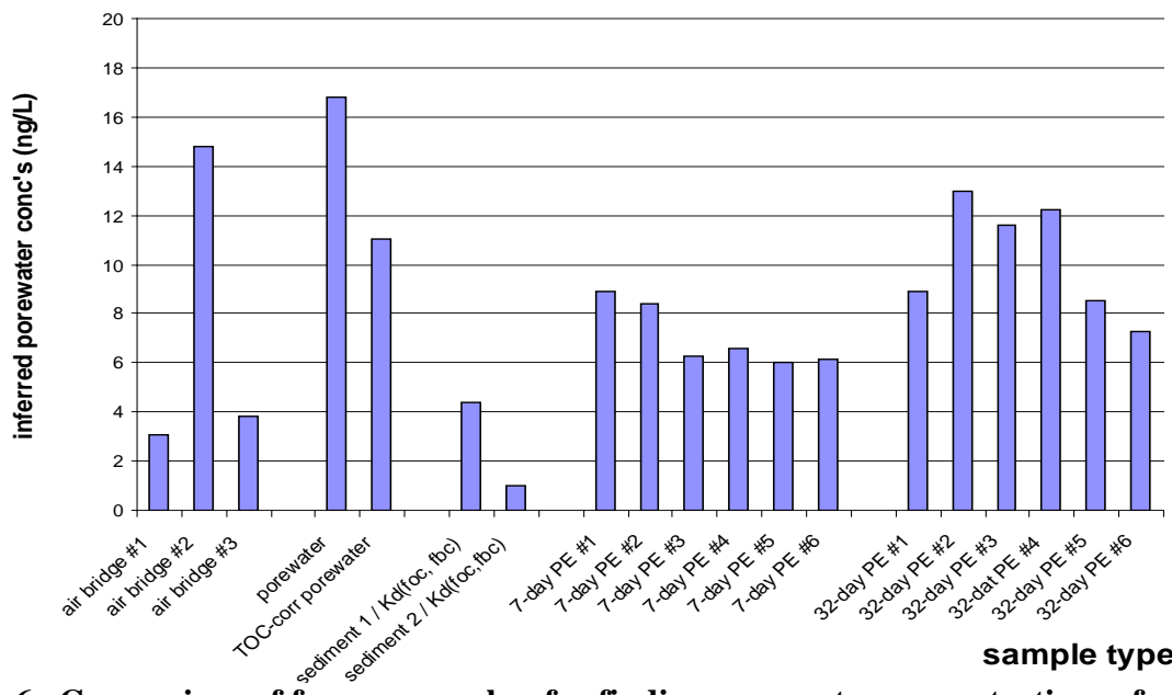
Figure 6. Comparison of four approaches for finding pore water concentrations of pyrene in Hunters Point sediments: (a) three air bridges, (b) pore water extraction, without and with correction for colloids, (c) sediment extractions, normalized with sorption coefficients estimated without and with consideration of black carbon presence, (d) six PE strips incubated in the sediment for 7 days and normalized by K_{pew} (pyrene) and (e) six PE strips incubated in the sediment for 32 days and normalized by K_{pew} (pyrene).
