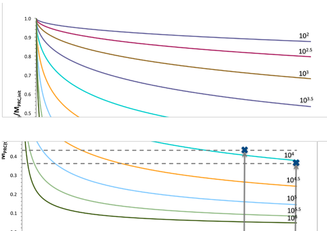
Figure 11. Measured fractional losses ( M_{\text{PRC}(t)}/M_{\text{PRC,init}} ) of a PRC (d10-pyrene) from PE strips exposed to Island End sediments (60% porosity) for defined times (setting the dimensionless time parameter, T = D_{\text{PE}} \cdot \text{time} / \text{PE thickness squared} ). A 25 \mu\text{m} thick PE was exposed for 3 days ( T=50 ) resulting in 36% loss, while a 51 \mu\text{m} thick PE was exposed for 10 days ( T=41 ) and had 43% loss. The intersections of these ( T, M_{\text{PRC}(t)}/M_{\text{PRC,init}} ) on this “type-curve” plot enables the K_d value for pyrene in this sediment to be estimated (here, 10^{4.0} and 10^{3.9} , respectively) and this is done for each PRC used in the PE strips. The resultant K_d(\text{PRC}) values are then used to establish a relationship between the analytes’ values of \log K_d and \log K_{ow} : \log K_d = 1.4 \times \log K_{ow} - 2.7 . Subsequently, this relationship is then used to estimate site-specific K_d values for other compounds of the same class.
