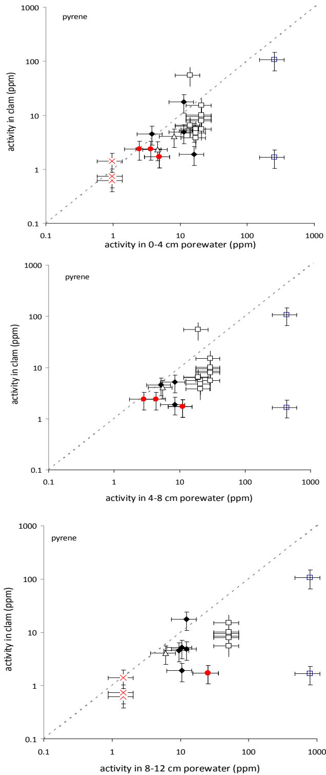
Figure 13. Pyrene chemical activities (ppm) at three depths (0-4, 4-8, and 8-12 cm) inferred from PE passive samplers versus activities found in soft-shell clam tissues from six sites near Boston, MA. Average ratios at 0-4 cm were 67%, at 4-8 cm were 48%, and 8-12 cm were 36%.
