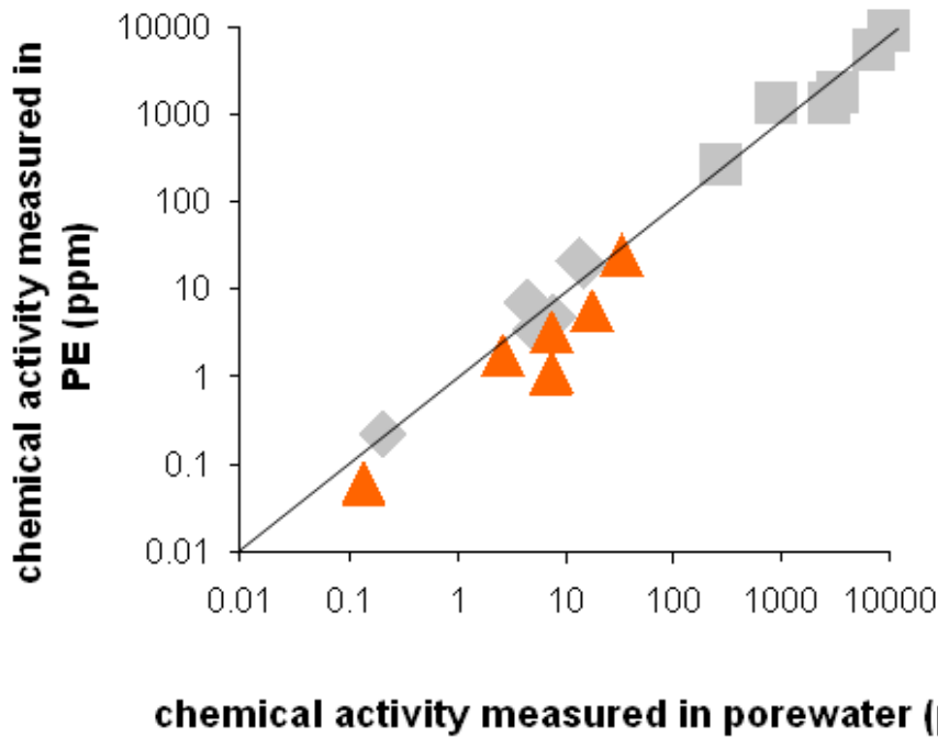
Figure 9. Comparison of PE-inferred pore water concentrations of six PAH when PE strips were deployed for 1 week in the field (orange symbols) with corresponding pore water concentrations measured in cores retrieved by divers near the PE incubation position. Gray symbols show results for the same PAH using sediments from other harbor sites in the laboratory for comparison.
