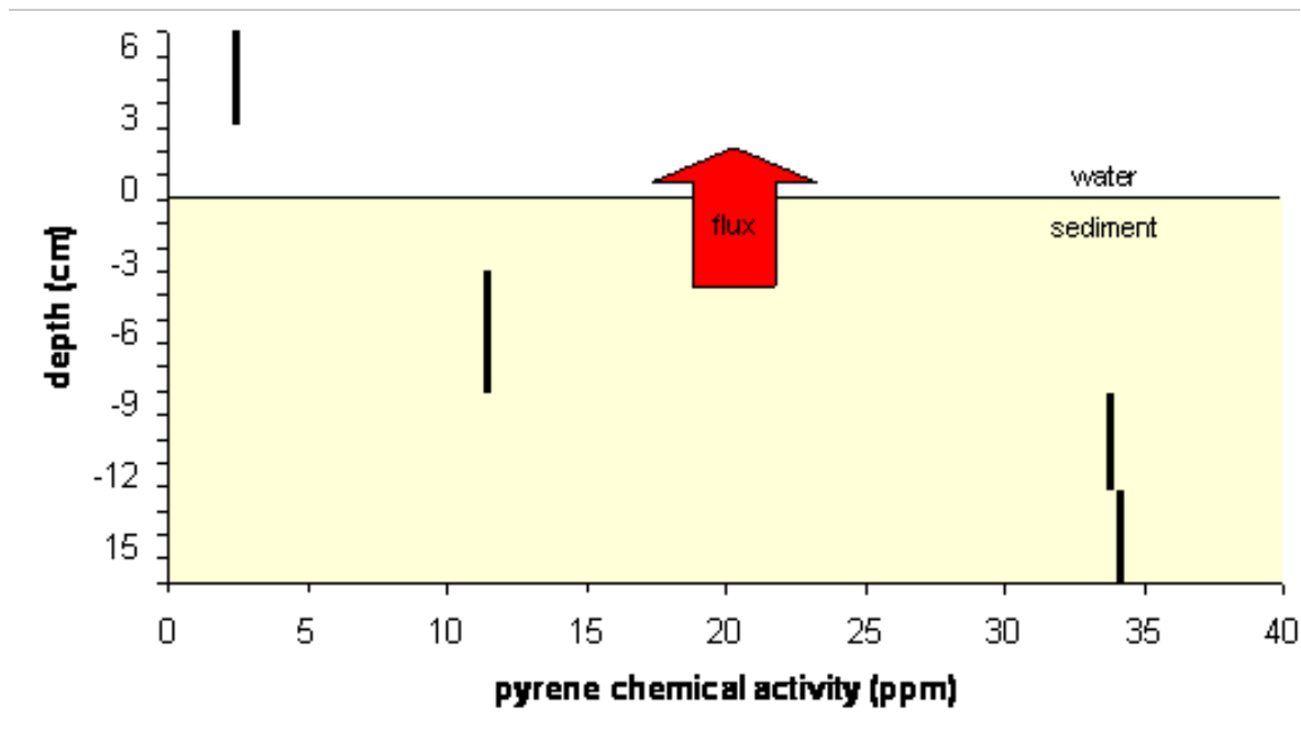
Figure 10. Profile of pyrene activities (= pore water concentration normalized by pyrene's liquid solubility of 900 ug/L) across the sediment-water interface for a site in Boston Harbor. Values were deduced from a polyethylene strip inserted ~20 cm into the bed but still have ~6 cm above the bed-water interface.
