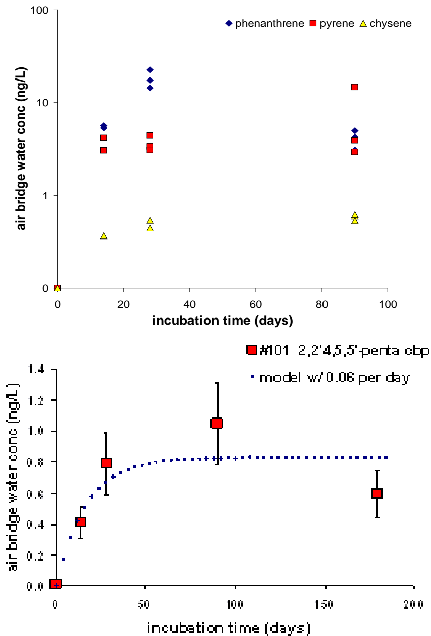
Figure 4. Example time courses of air bridge results showing build up of representative PAH (upper panel), and a representative PCB, 2,2',4,5,5'-pentachlorobiphenyl (lower panel), in the initially pure water outside the sample-containing beaker. The PAH case involved use of the coal-tar-contaminated sediment from the Island End site in Boston Harbor, while the PCB case involved Hunter's Point sediment.
