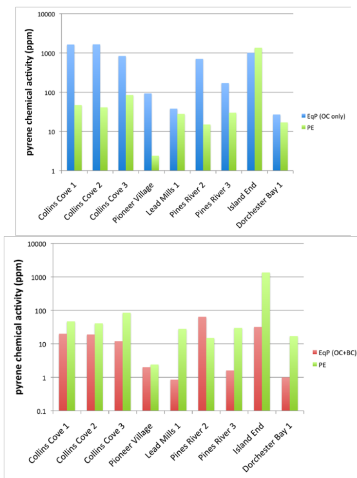
Figure 15. Comparison of pyrene's chemical activities (pore water concentration normalized by pyrene's liquid solubility) measured in pore waters using PE passive samplers (green bars) and calculated using an EqP model (upper panel) assuming only equilibrium absorption into organic carbon (i.e., K_d = f_{oc}K_{oc} ) and (lower panel) considering sorption to both organic carbon and black carbon (i.e., K_d = f_{oc}K_{oc} + f_{bc}K_{bc}C_w^{n-1} ).
