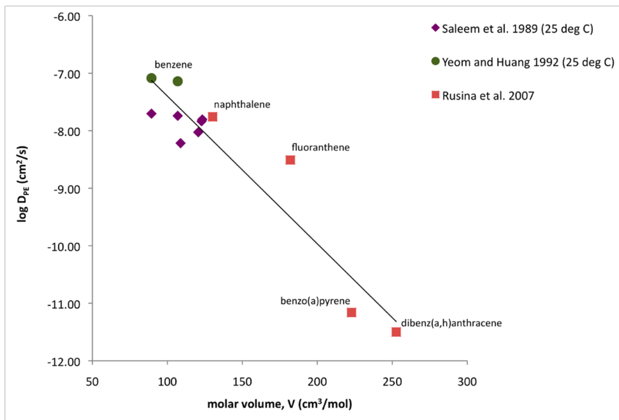
Figure 2. Published log D_{PE} values versus molar volumes ( V ) for ten aromatic compounds. The best-fit log-linear relationship, \log D_{PE} = -0.026 \times V - 4.8 , was used to estimate D_{PE} for PAH in this study.
