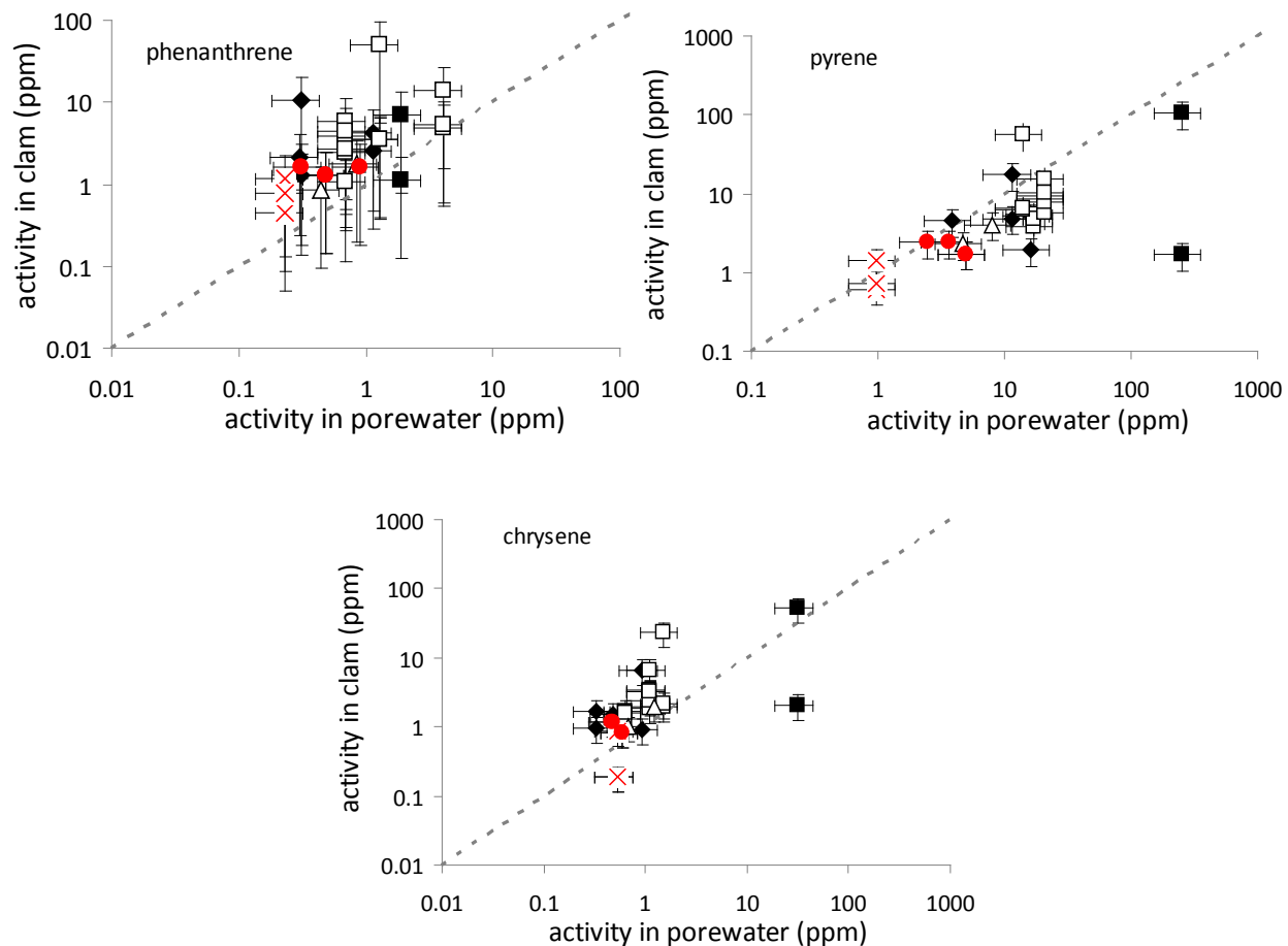
Figure 14. Chemical activities of three PAH measured in pore waters (0-4 cm depth) using PE passive samplers and in clam tissues at six sites near Boston, MA.
