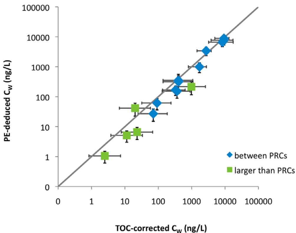
Figure 12. Use of a few PRC to adjust measured PE loads of PAH to values expected at sediment-PE equilibration for two sets of target contaminants (a) those that exhibit partitioning properties between those of the three ^{13}\text{C} -labeled PRC (phenanthrene, pyrene, and chrysene) and (b) those that have partitioning properties outside those of the three PRC. The resultant PRC-corrected estimates are then normalized using K_{pew} values to deduce C_{pw} and compared to pore water concentrations found by solvent extraction and corrected for sorption to colloidal organic carbon for Island End sediments. The 1:1 line is shown, and the error bars represent \pm 1\sigma .
