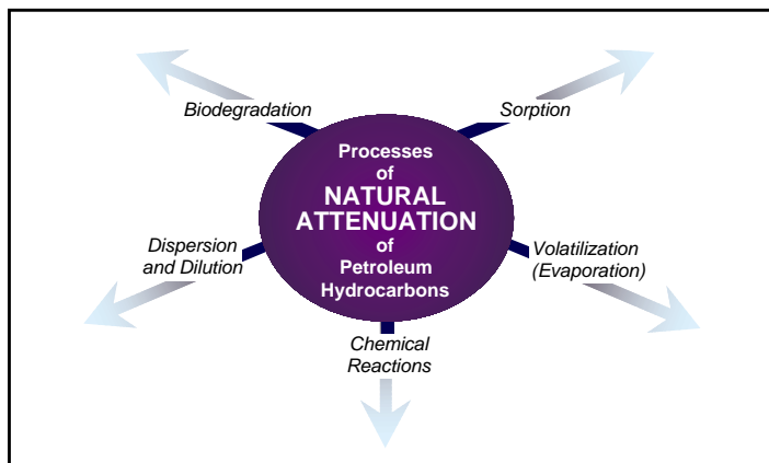
Figure 1. Processes of natural attenuation of petroleum hydrocarbons.
