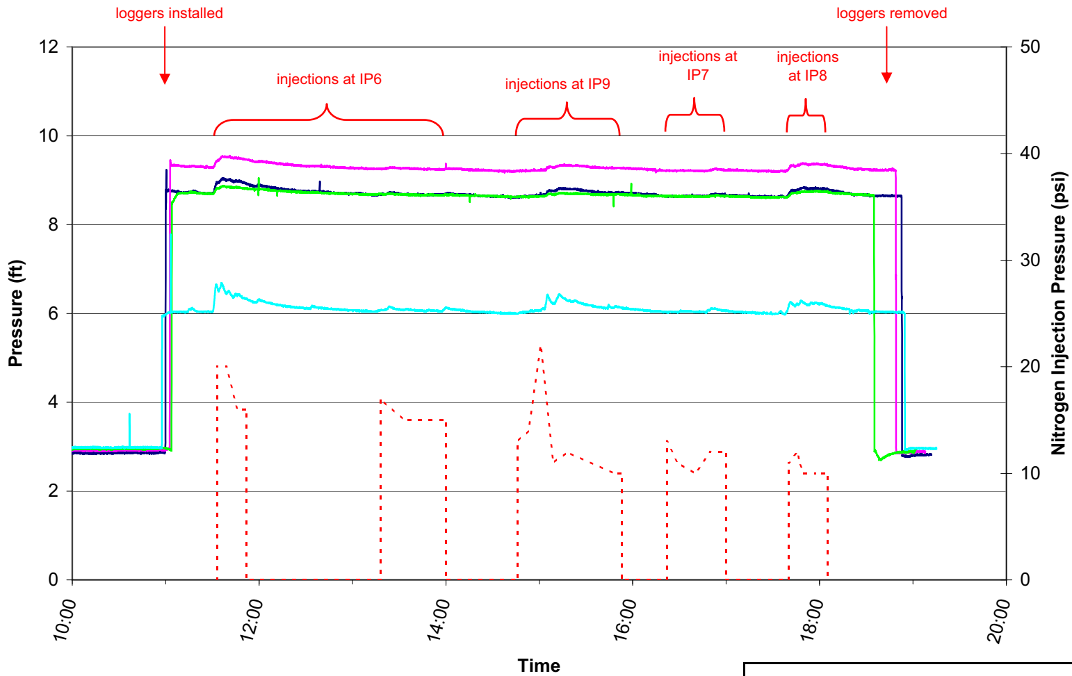
Down-Well and Nitrogen Injection Pressures - Oct 15, 2006 Site 45, Parris Island MCRD, Parris Island, SC
