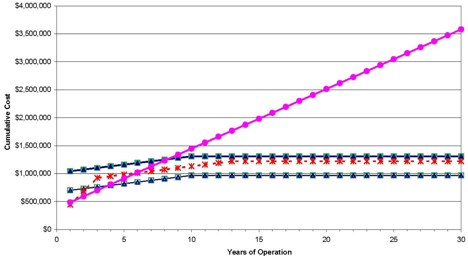
Cumulative Costs for EZVI, ISCO and P&T Alternatives Site 45, Parris Island MCRD, Parris Island, SC
