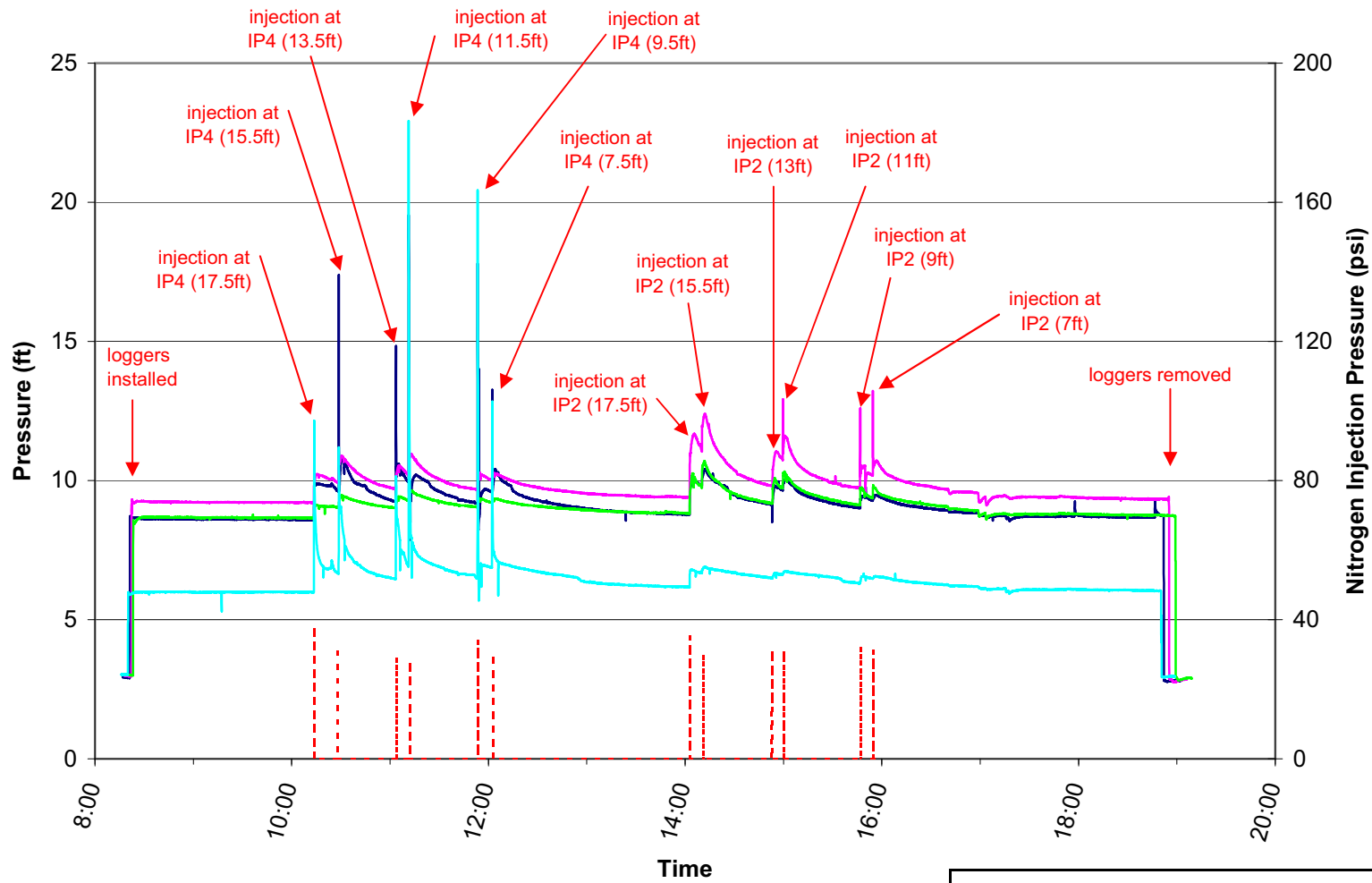
Down-Well and Nitrogen Injection Pressures - Oct 16, 2006 Site 45, Parris Island MCRD, Parris Island, SC
