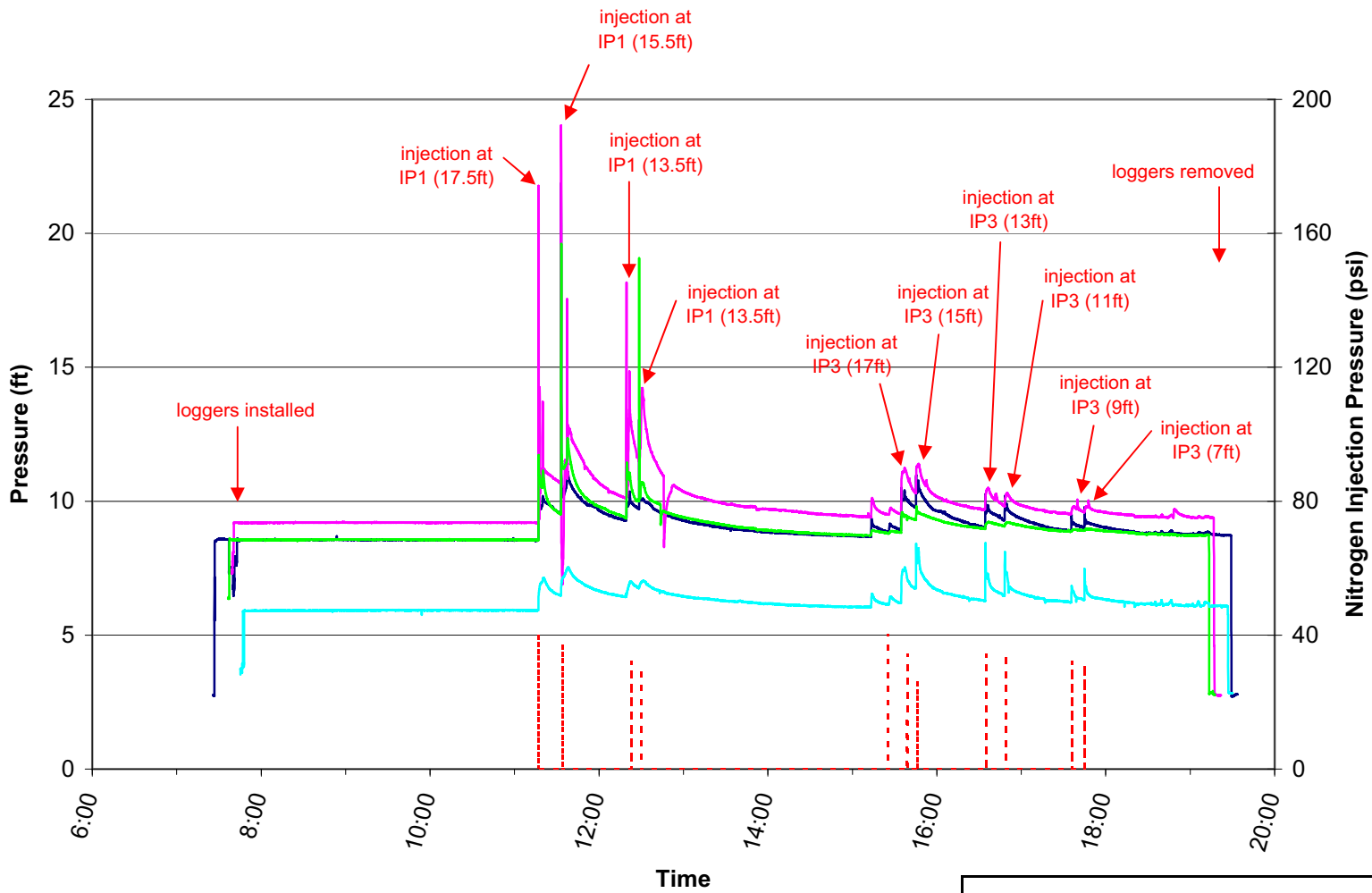
Down-Well and Nitrogen Injection Pressures - Oct 14, 2006 Site 45, Parris Island MCRD, Parris Island, SC
