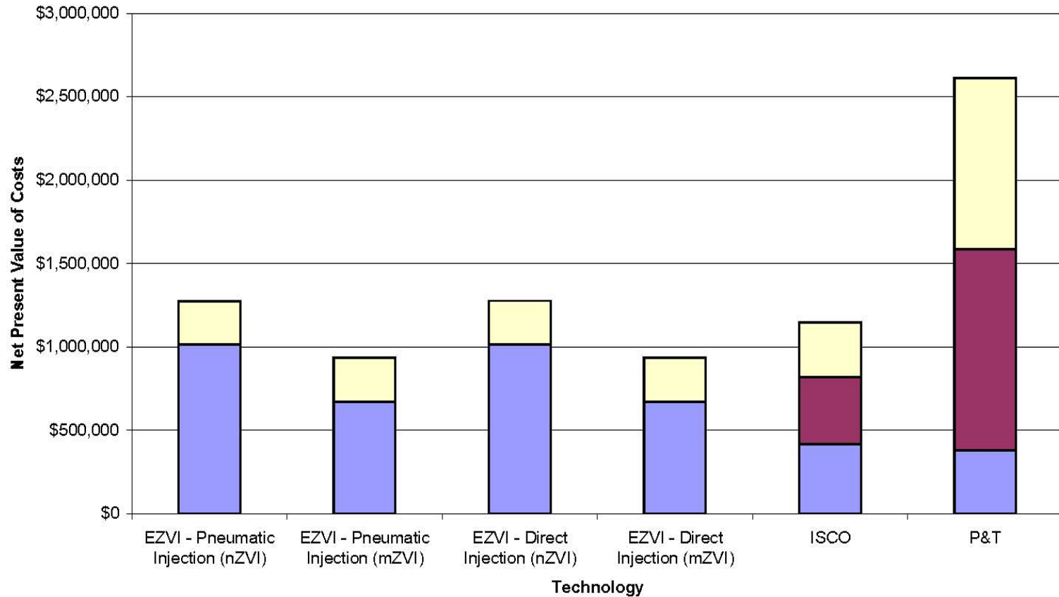
NPV of Costs for EZVI, ISCO and P&T Options Site 45, Parris Island MCRD, Parris Island, SC
