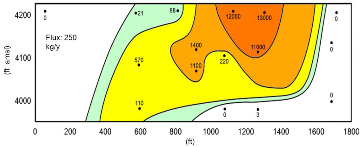
Figure 5C: Vertical Groundwater Concentration Contour Plot Along Transect A-A': Event 3 – September 2010: PCE Equivalence concentration values in µg/L
