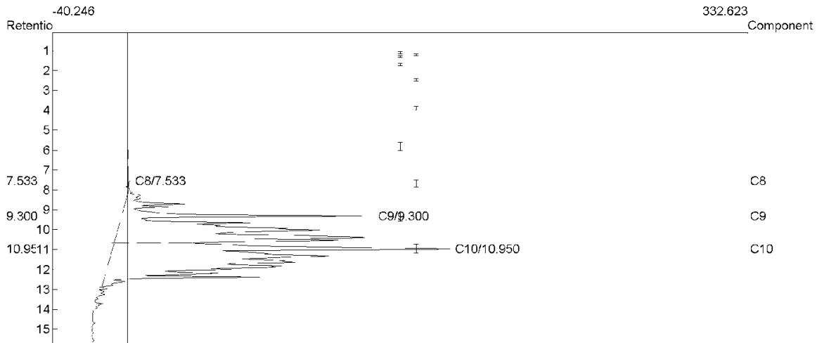
Chromatogram for direct injection of LNAPL from ML6 – 9ftbgs: Event 1: October 16-26, 2008
