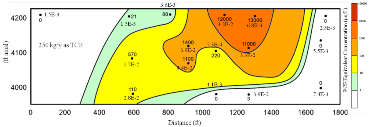
Figure 6.13. Site 3 event 3 groundwater transect contour plot with collocated values of concentration as TCE ( \mu\text{g/L} ) (upper values; \mu\text{g/L} ) and hydraulic conductivity (lower values in scientific notation; cm/sec). Mass discharge of 250 kg/y as TCE.
