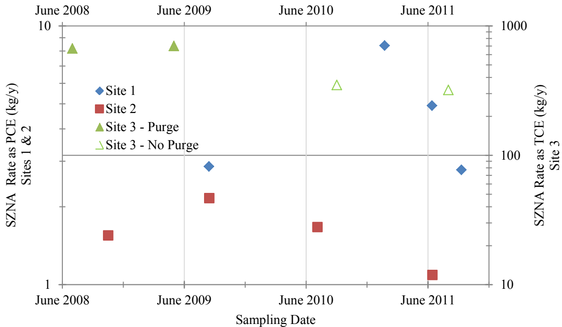
Figure 6.19. Averaged CAH dissolved contaminant discharge rates vs. time for three sites sampled. Note: Site 1 and 2 and displayed on the left y-axis and Site 3 on the right y-axis.
