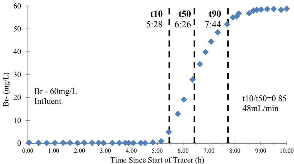
Figure 5.8: Bromide tracer plot.
