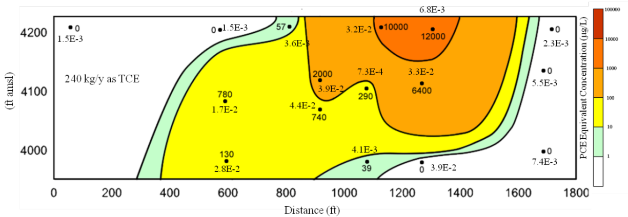
Figure 6.14. Site 3 event 4 groundwater transect contour plot with collocated values of concentration as TCE ( \mu\text{g/L} ) (upper values; \mu\text{g/L} ) and hydraulic conductivity (lower values in scientific notation; cm/sec). Mass discharge of 240 kg/y as TCE.
