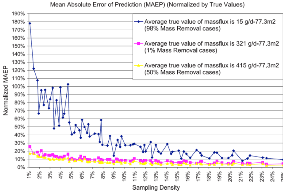
Figure 4.3: Normalized error of predicted mass discharge vs. sampling density (from Li et al., 2007); MAEP = (estimated discharge – true discharge)/true discharge.
