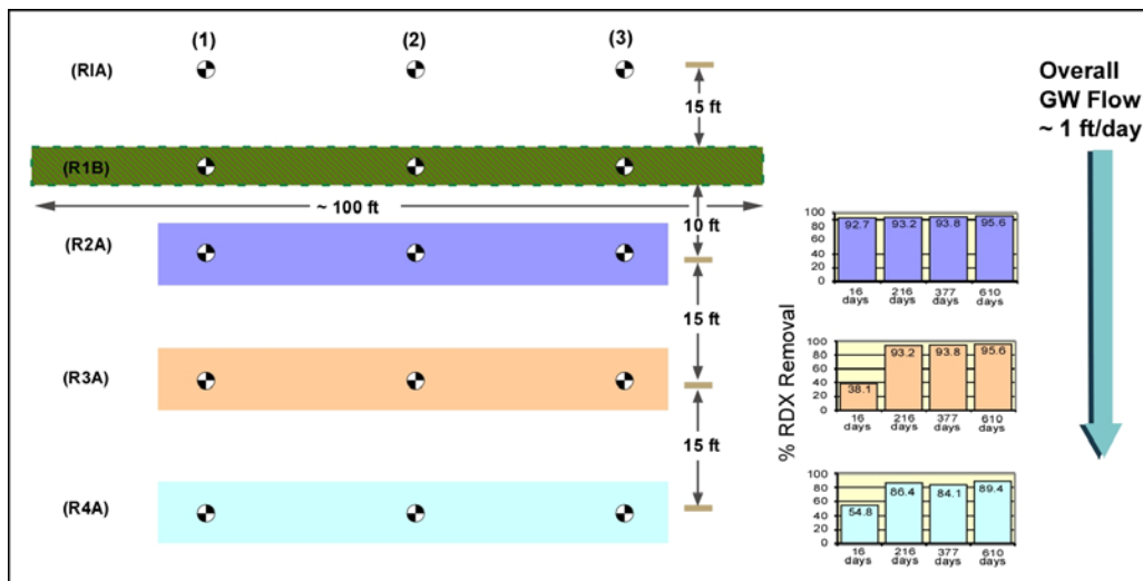
Figure 23. Row-averaged RDX Removal Over the Course of the Field Demonstration.
