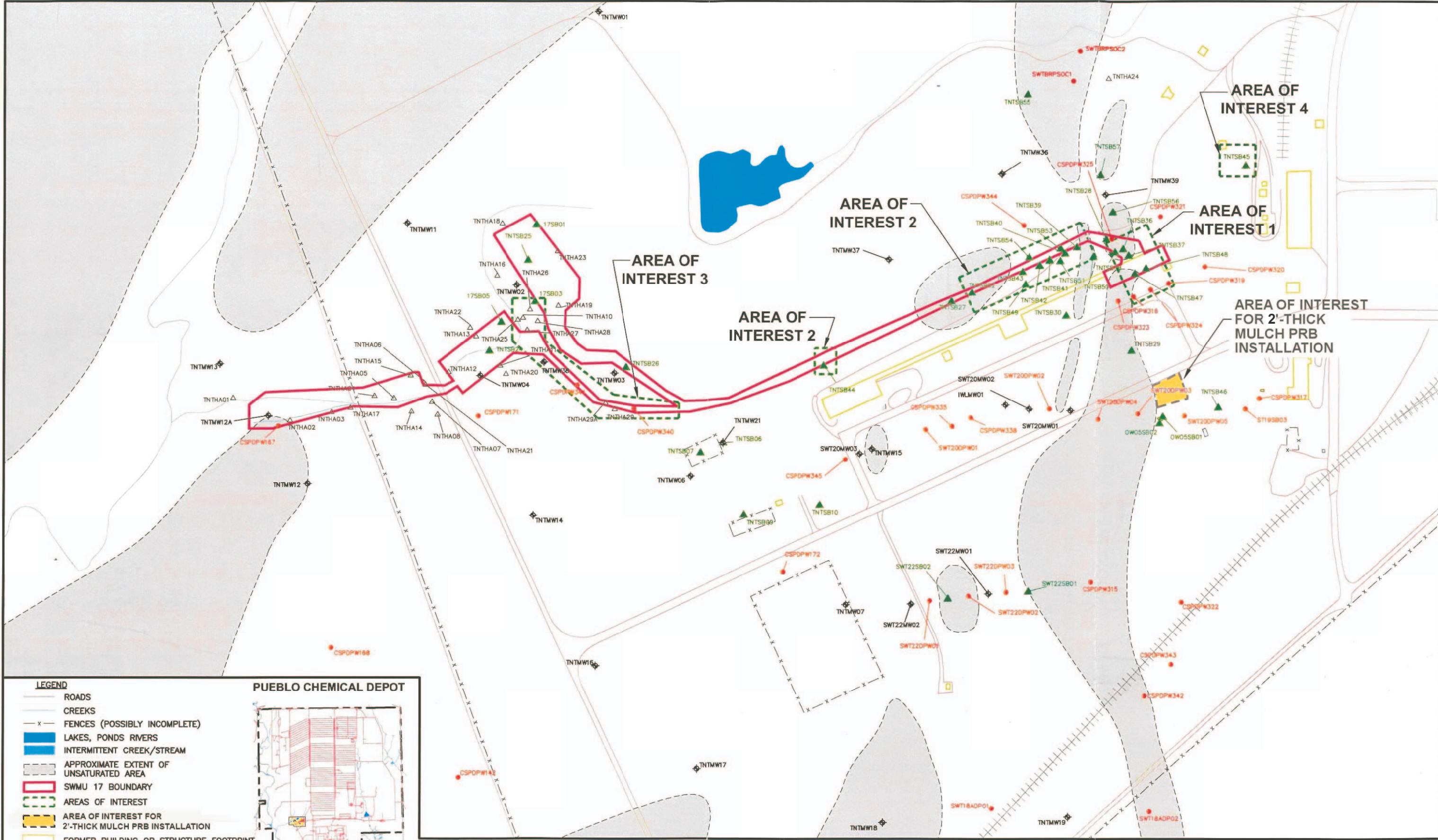
FIGURE 10 LOCATION OF MULCH PRB PUEBLO CHEMICAL DEPOT PUEBLO, COLORADO DEC. 2004 62317
