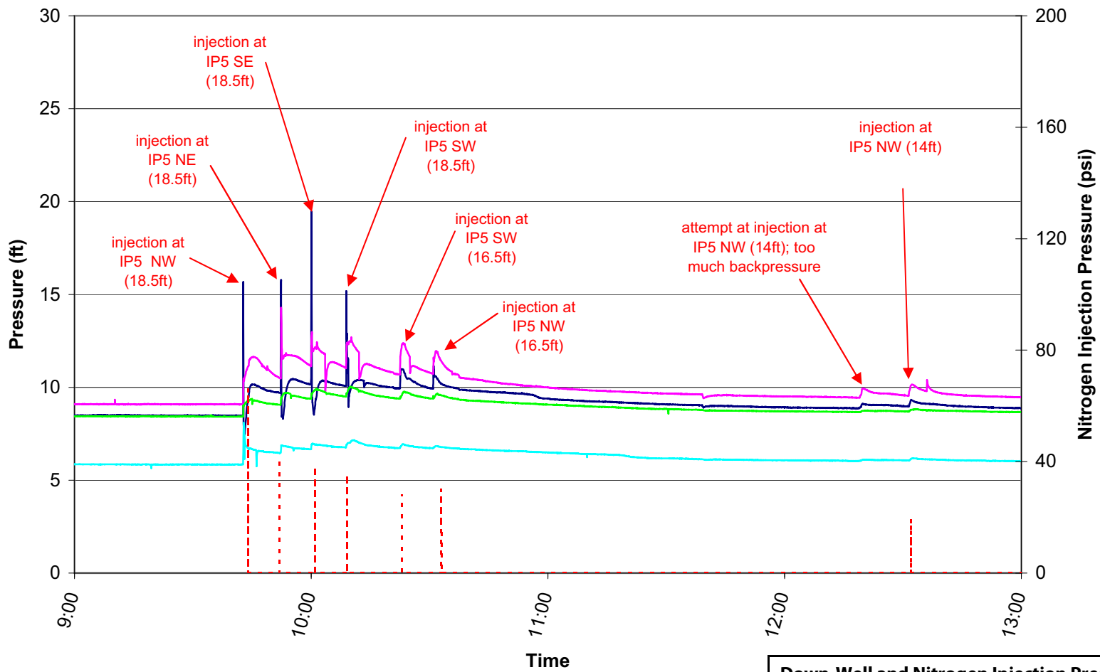
Down-Well and Nitrogen Injection Pressures - Oct 17, 2006 (09:00 - 13:00) Site 45, Parris Island MCRD, Parris Island, SC
