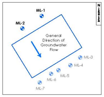
VOC Trends in Upgradient Wells (ML-1 and ML-2) Site 45, Parris Island MCRD, Parris Island, SC
